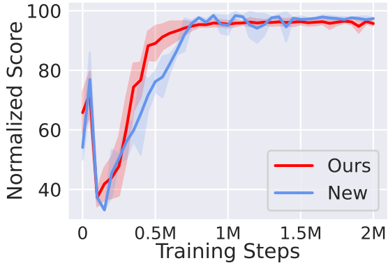
walker2d-medium-v2-v2
