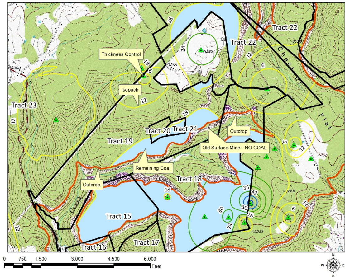
New Haven/Bellwood Tract 19 - Pocahontas No. 7 Seam
