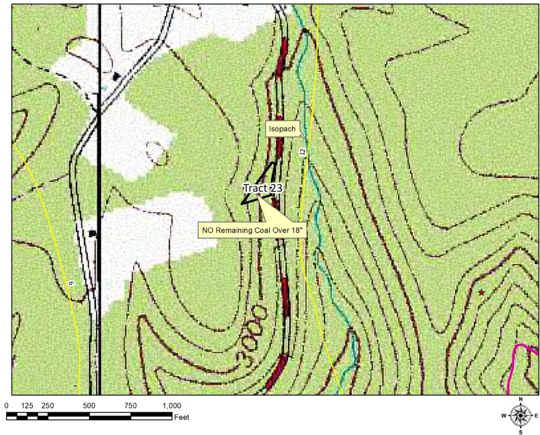
Tract 23 – Pocahontas No 9 Seam – NO remaining coal of 18” thick.
