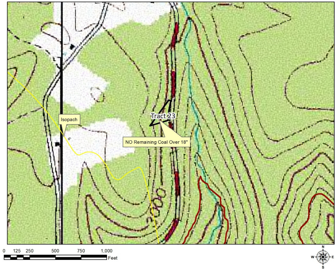
Tract 23 – Fire Creek Seam – NO remaining coal of 18” thick.
