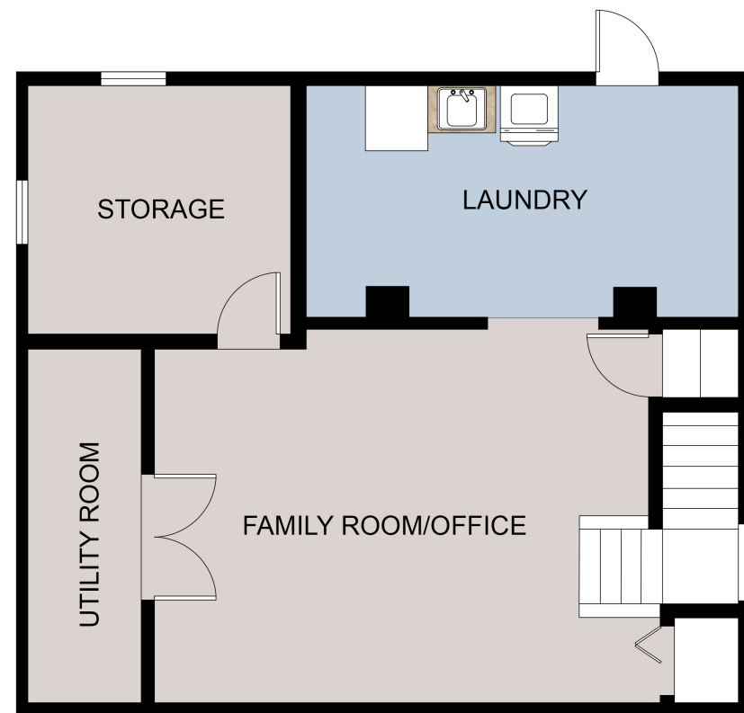
BASEMENT
