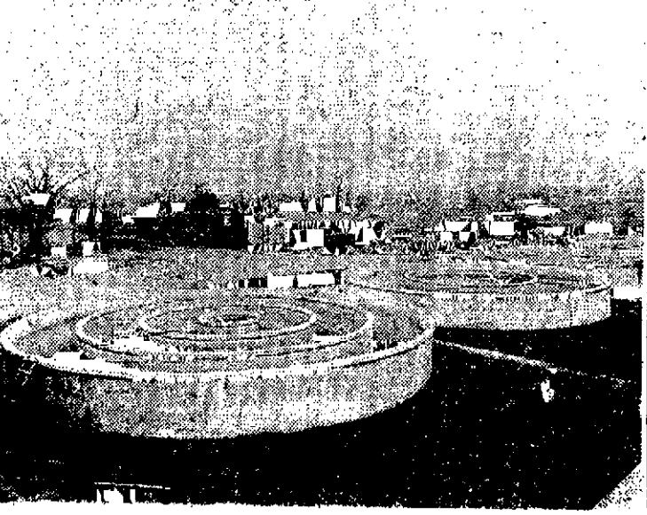
The sponge and coke basins at Lancaster, through which the water to be filtered first passes and in which the added chemicals are supposed to be thoroughly mixed.
